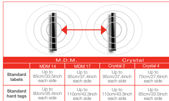
Detection Area on each side of pedestals
